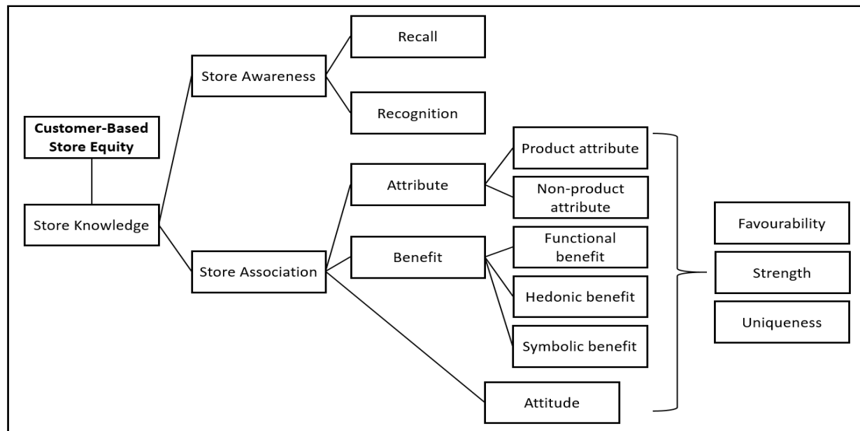
Figure 1 CBSE Model
